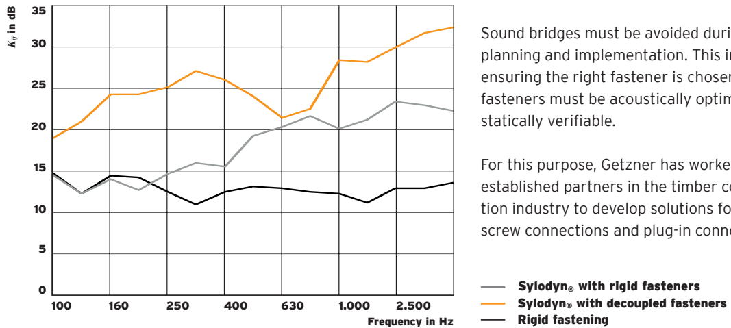
Abb. 2: K_{12} Plot for a T-joint with Sylodyn® and elastic fastener, Sylodyn® with rigid fastener and without elastomer intermediate layer
