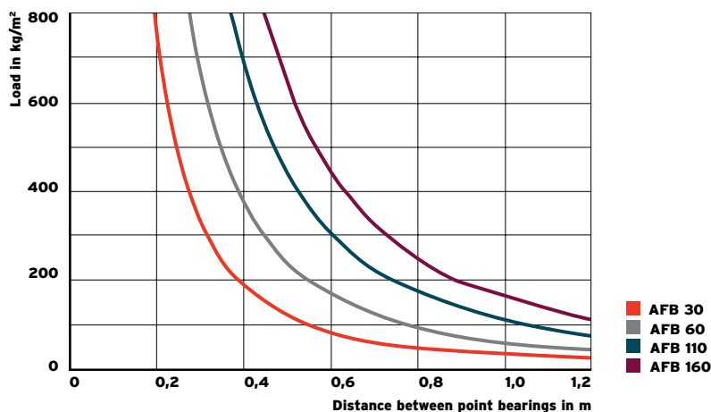
Fig.2: Distance between point bearings with different loads
